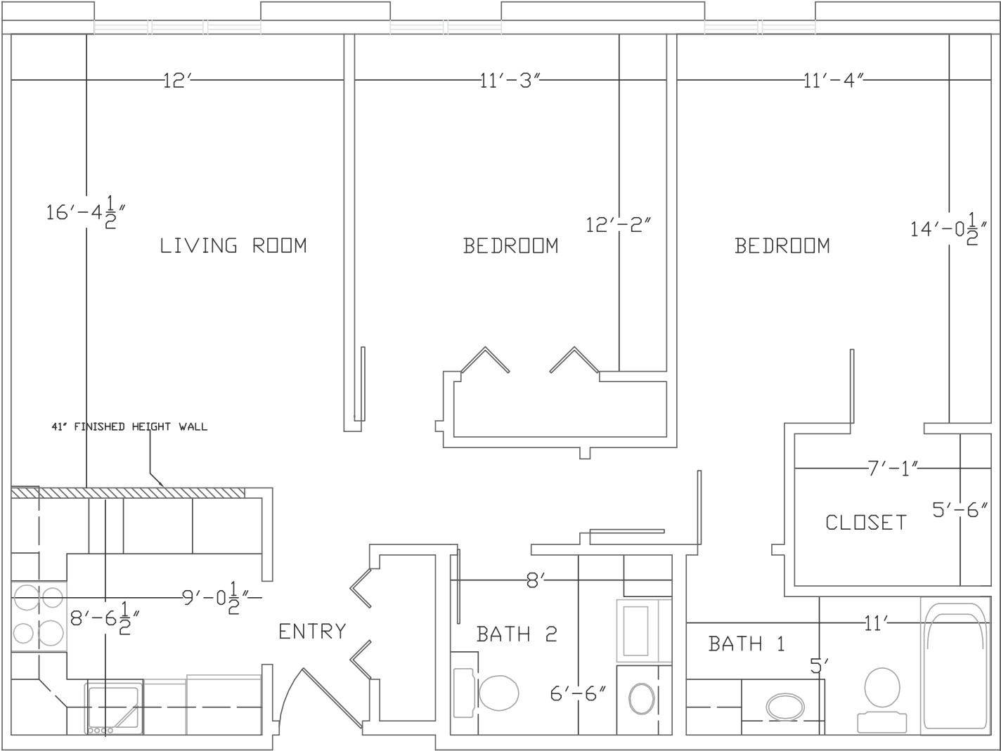
Two Bedroom 947 SQ. FT.
